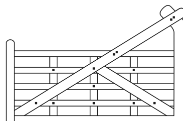
Curved Heel Gate
